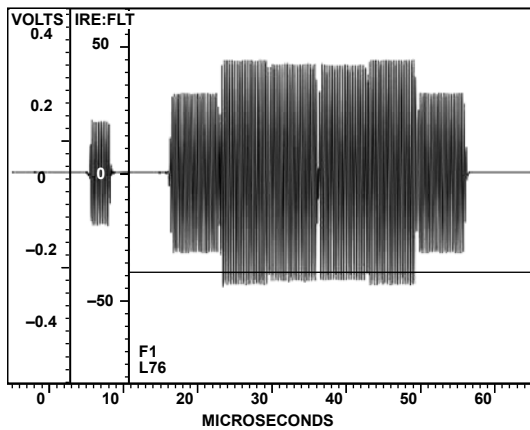
Figure 131. NTSC Luma
