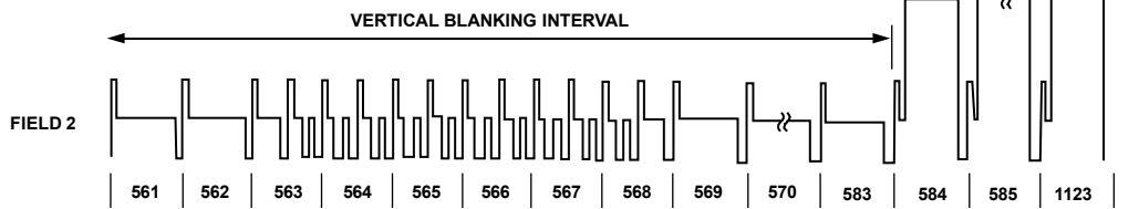
Figure 141. SMPTE 274M (1080i)
