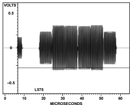
Figure 134. PAL Luma
