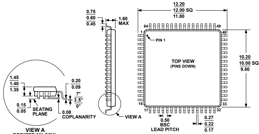
Figure 142. 64-Lead Low Profile Quad Flat Package [LQFP]
